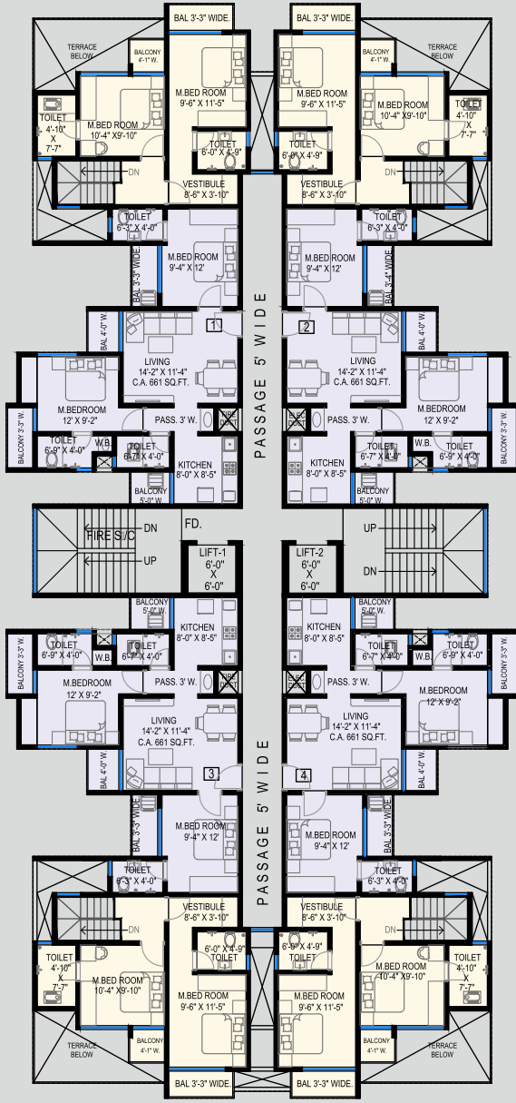
TOWER-1 2ND, 4TH, 6TH, 8TH, 10TH, 12TH FLOORS PLAN
