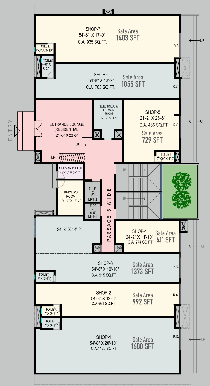
TOWER-2 GROUND FLOOR PLAN
