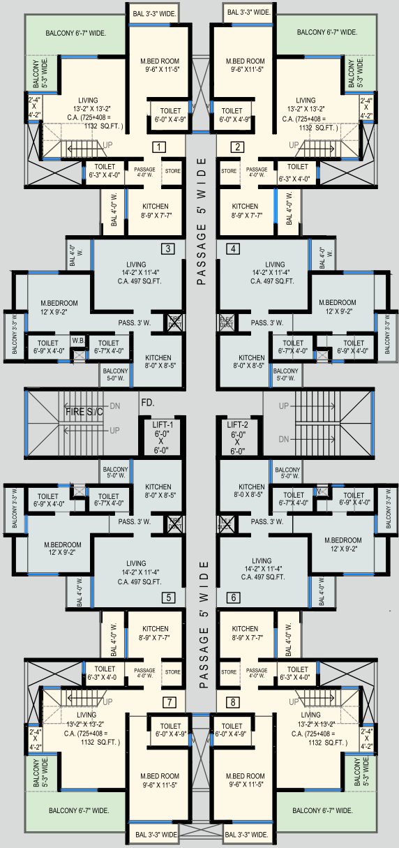
TOWER-1 3RD, 5TH, 7TH, 9TH,11TH FLOORS PLAN
