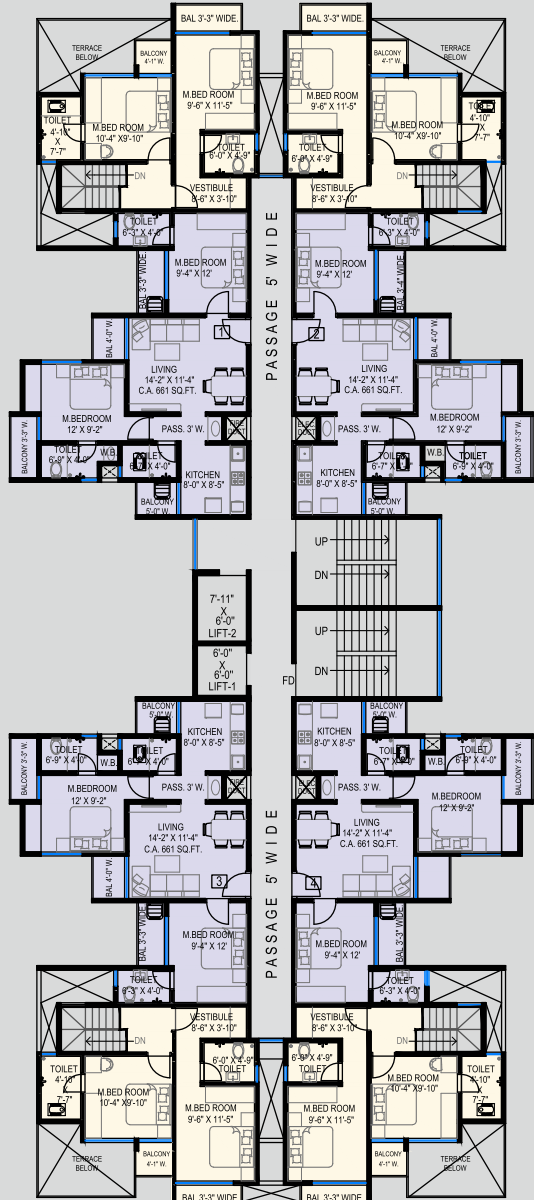
TOWER-2 2ND, 4TH, 6TH, 8TH, 10TH, 12TH FLOORS PLAN
