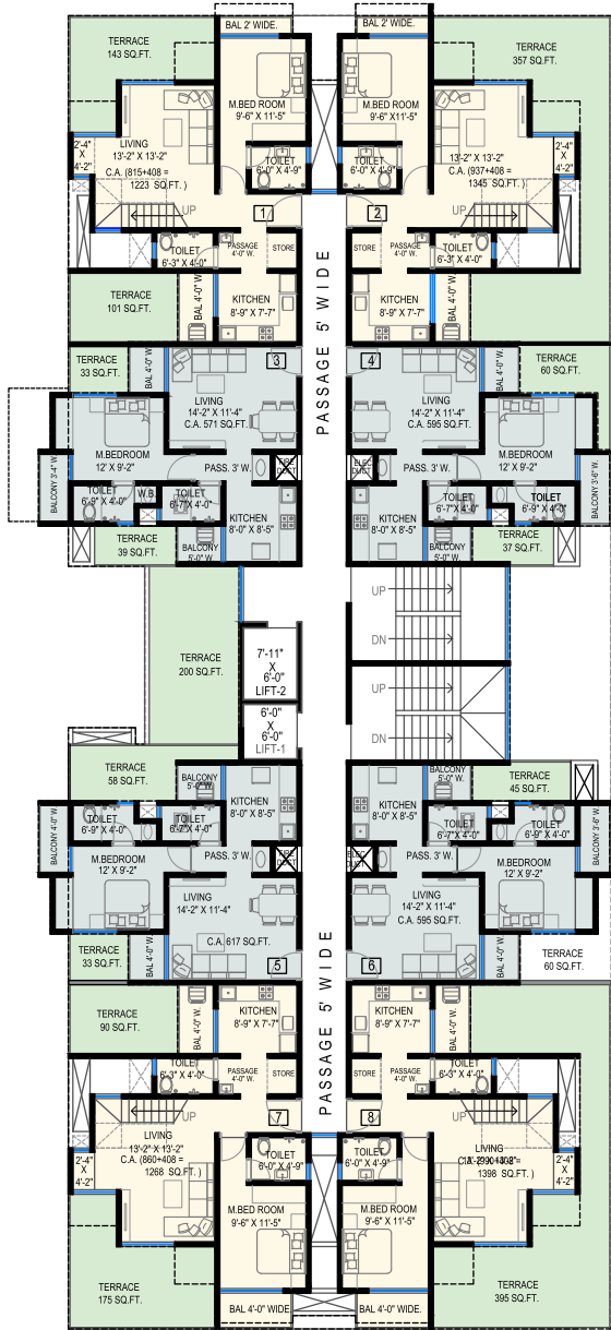
TOWER-2 1ST FLOOR PLAN
