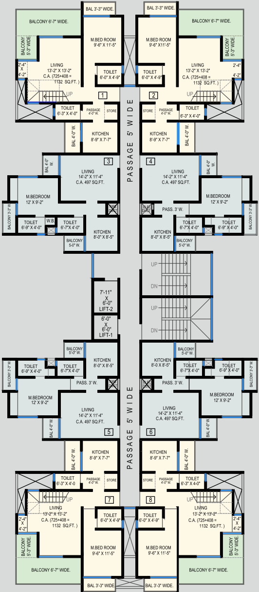
TOWER-2 3RD, 5TH, 7TH, 9TH, 11TH FLOORS PLAN
